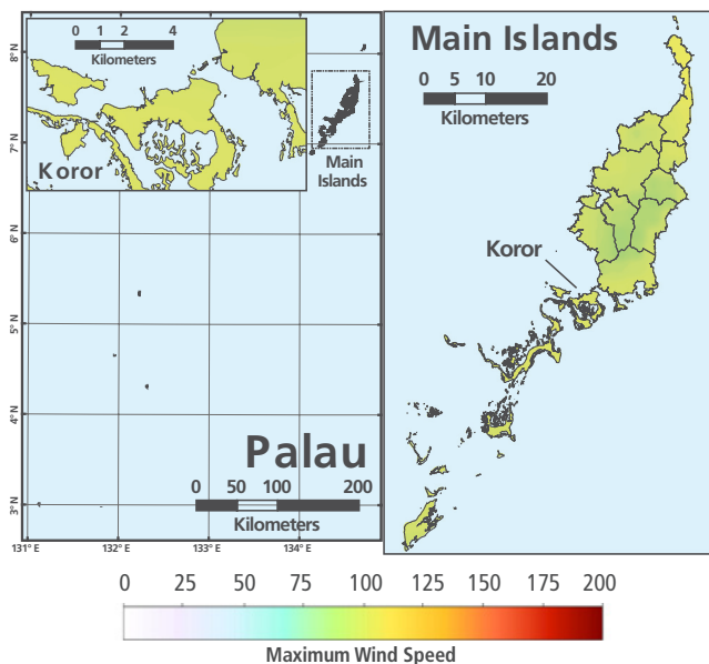
Figure 4: Maximum 1-minute sustained wind speed (in miles per hour) with a 40% chance to be exceeded at least once in the next 50 years.(100-year return period).
